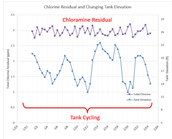
With the Monoclor® RCS system, the Landmark Tank maintained the chloramine residual set-point
